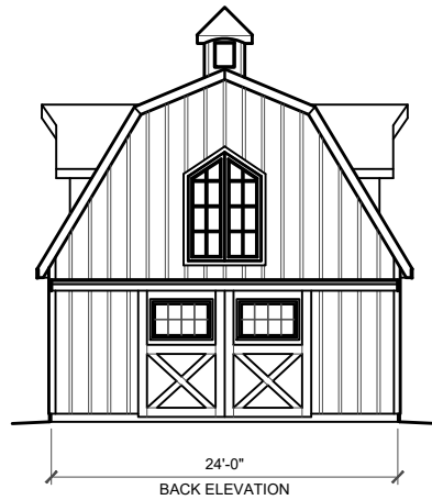
BACK ELEVATION
