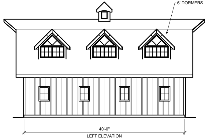
LEFT ELEVATION
